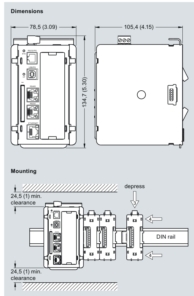
SITRANS RD500 dimensions
