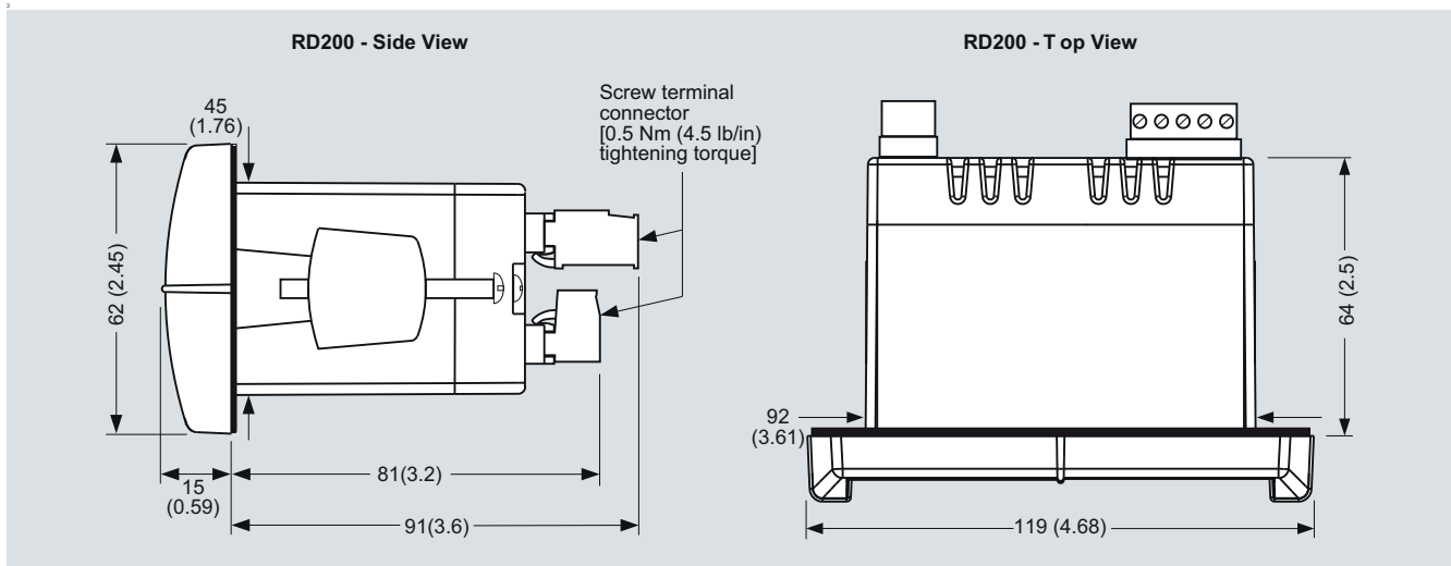
SITRANS RD200 dimensions
