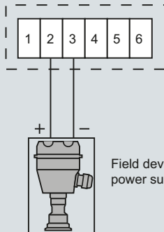
Connection of a four-wire field device
