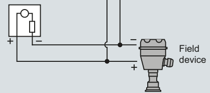
Connection of adapter parallel to wired 4 to 20 mA communication
