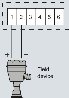
Connection of a two-wire field device, power supply provided by adapter
