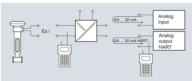
SITRANS I200 output isolator, function block diagram
