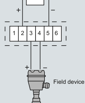
Connection of a two-wire field device with external power supply
