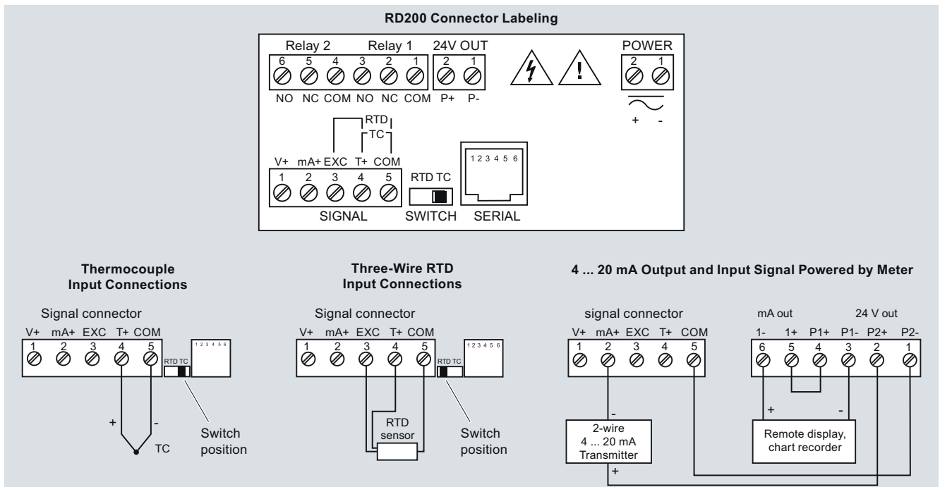
SITRANS RD200 connections
